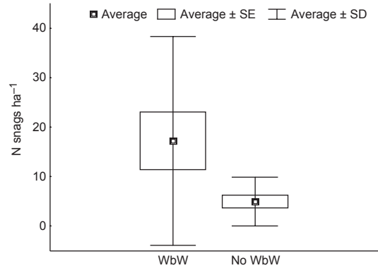
Fig. 2. Average number of snags (> 20 cm DBH) on studied samples.
