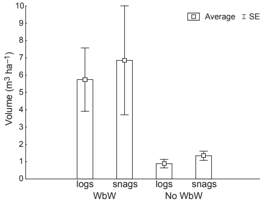
Fig. 3. Average volume of downed logs on studied samples.
