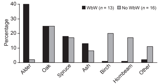
Fig. 4. Share of dead wood on studied plots according to tree species.
